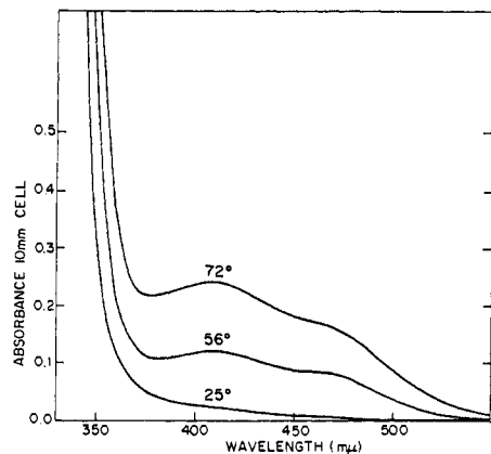
Figure 3. Optical spectra of 0.019 M Ni[P(O-p-tolyl)_3]_4 at various temperatures in benzene.
