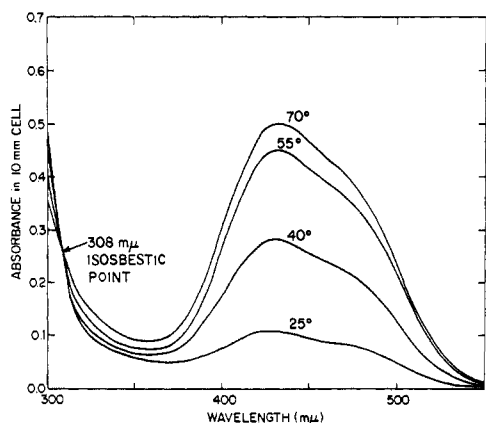
Figure 4. Optical spectra of 1.92 \times 10^{-4} M Ni[P(O-i-Pr)_3]_4 at various temperatures in benzene.
