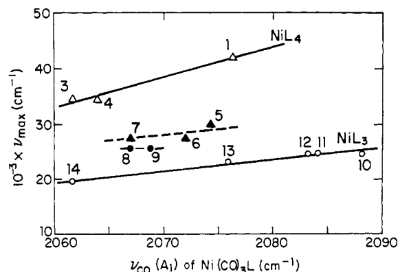
Figure 2. Frequency of longest wavelength electronic absorption maximum vs. A 1 stretching frequency of Ni(CO) 3 L from ref 33: Δ, NiL 4 without P-Ph; ▲, NiL 4 with P-Ph; ●, NiL 3 with P-Ph; ○, NiL 3 without P-Ph. The ligand numbers refer to Table IV.
