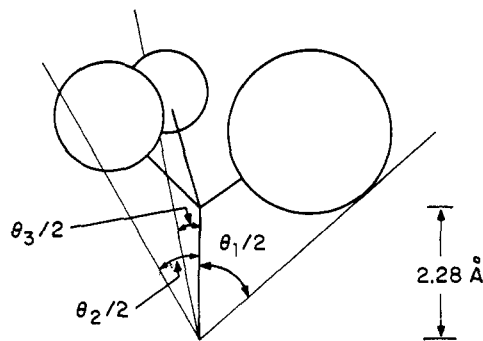
Figure 7. Method of measuring cone angles for unsymmetrical ligands.
