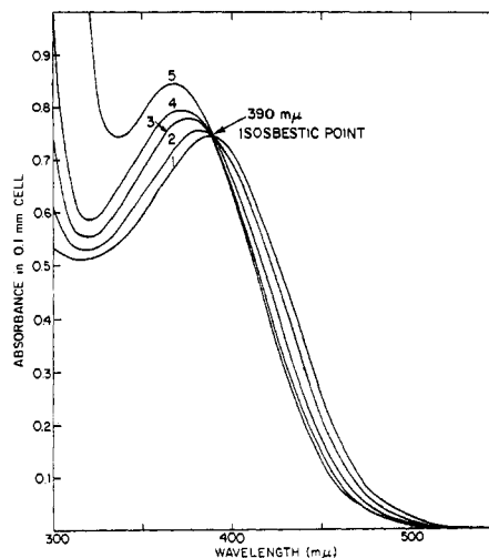
Figure 5. Optical spectra of 3.64 \times 10^{-3} M Ni[PMePh_2]_4 in benzene at 25^\circ with increasing concentrations of added PMePh_2 : (1) none; (2) 0.02 M ; (3) 0.05 M ; (4) 0.10 M ; (5) 2.0 M .
