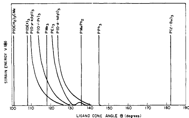
Figure 6. Strain energy in phosphorus ligand models as the ligand cone is compressed.
